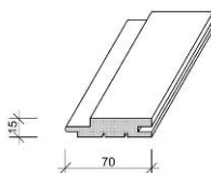
STS 15 x 70 mm
