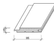
STS 15 x 95 mm
